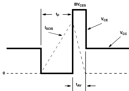
Figure 21. Energy Waveforms
