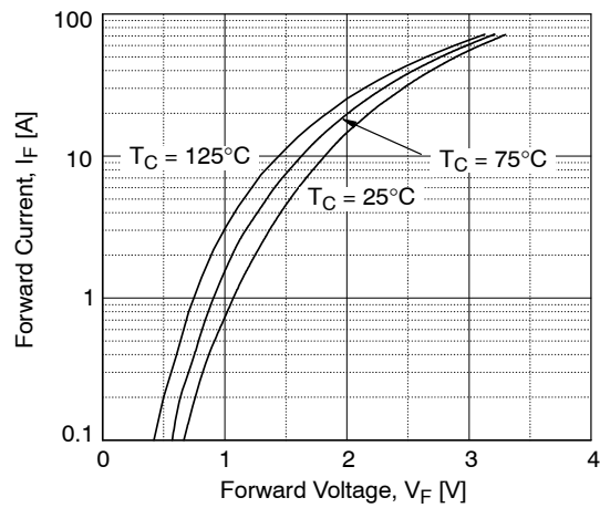
Figure 19. Forward Characteristics
