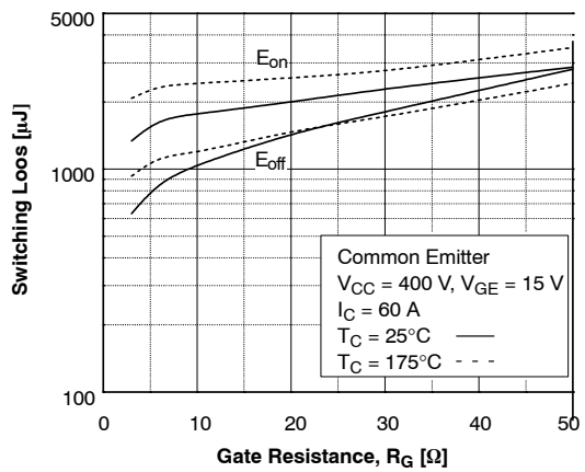
Figure 11. Switching Loos vs. Gate Resistance
