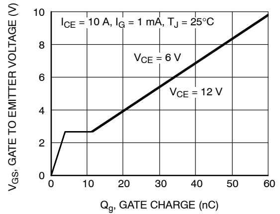
Figure 14. Gate Charge
