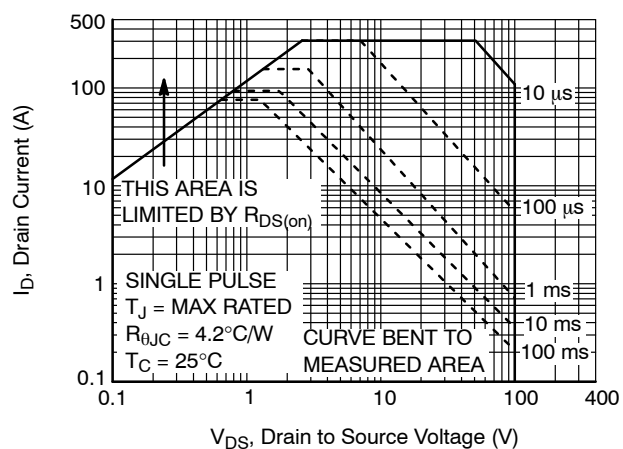
Figure 12. Forward Bias Safe Operating Area for FDPF8D5N10C
