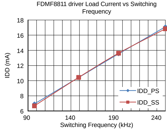
Figure 20. Driver Current per FDMF8811 vs. Switching Frequency
