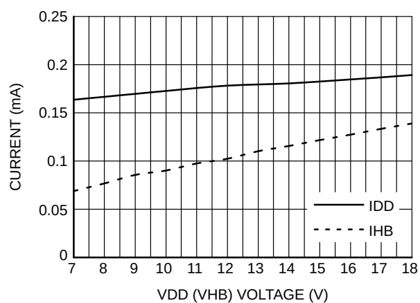
Figure 14. Driver Quiescent Current vs. V_{DD} ( V_{HB} )
