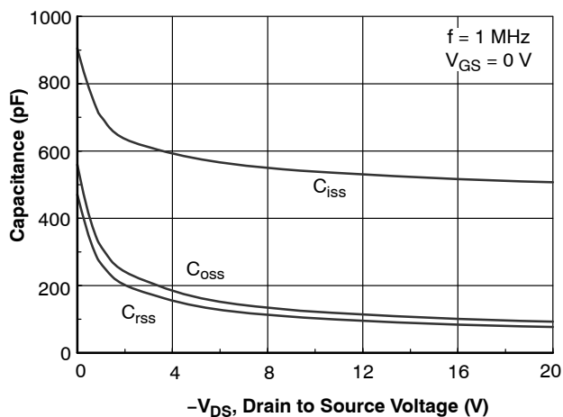
Figure 19. Capacitance Characteristics
