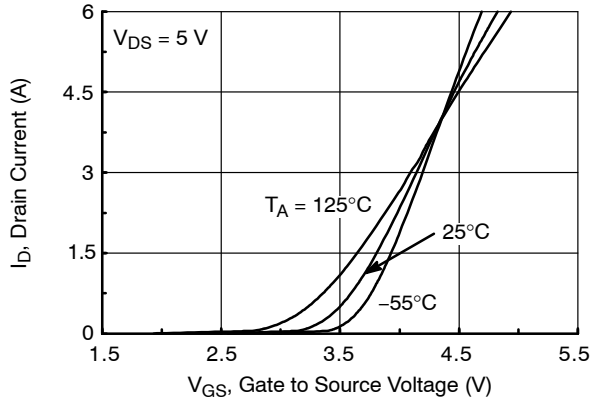
Figure 5. Transfer Characteristics
