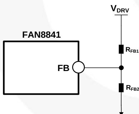
Figure 27. Feedback Circuit
