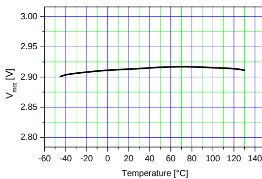
Figure 19. Maximum On-Time Voltage vs. Temp.
