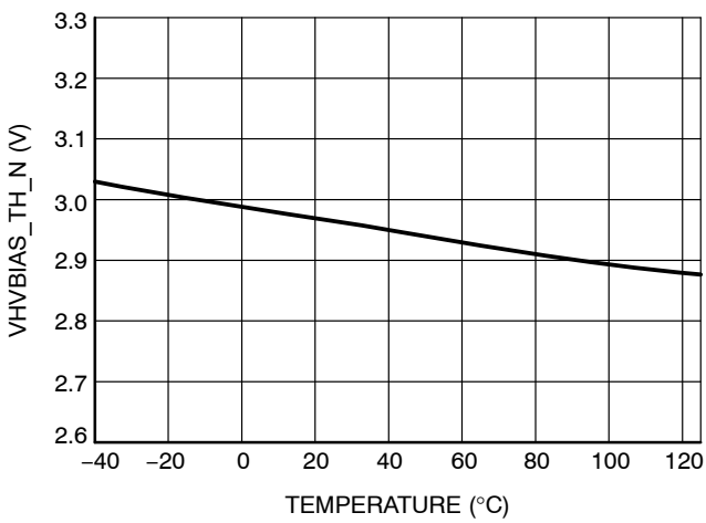
Figure 8. HVBIAS Falling Threshold vs. T
