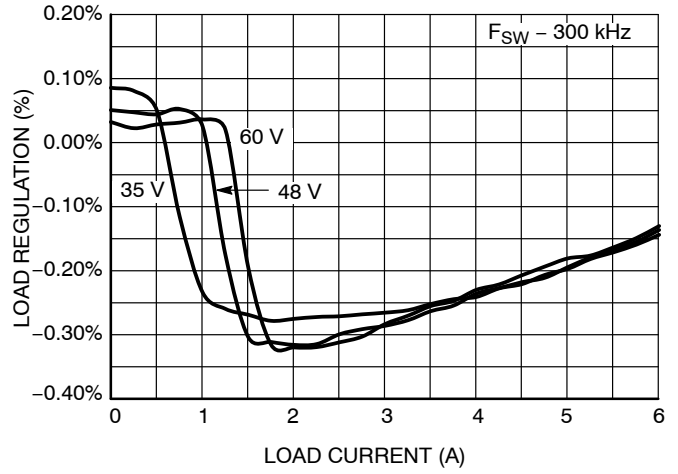
Figure 34. Load Regulation
