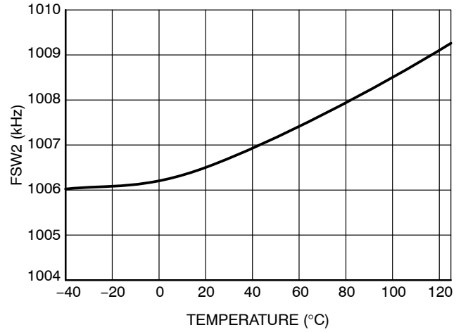
Figure 13. Switching Frequency vs. T at V_{HVBias} = 48\text{ V} and RT = 8.06\text{ k}\Omega
