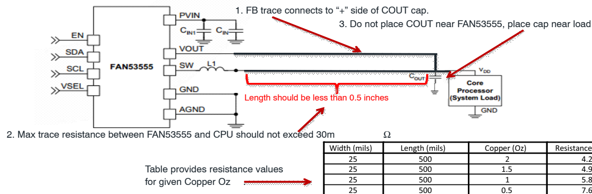
Figure 43. Remote Sensing Schematic
