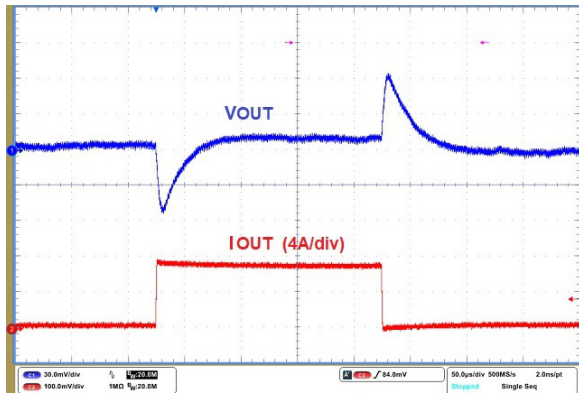
Figure 10. Load Transient 0–7.5 A, 10 A/μs
