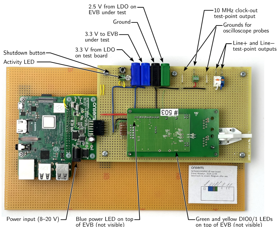
Figure 21. Test Board
