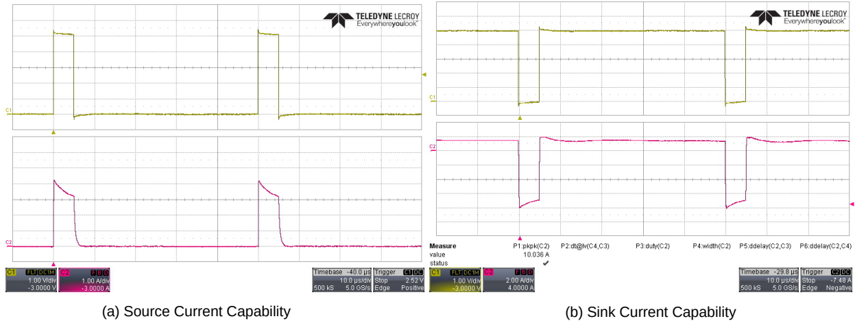
Figure 19. Experimental Waveforms of Current Driving Voltage
