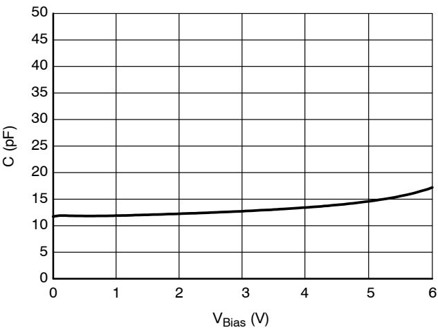
Figure 3. CV Characteristics
