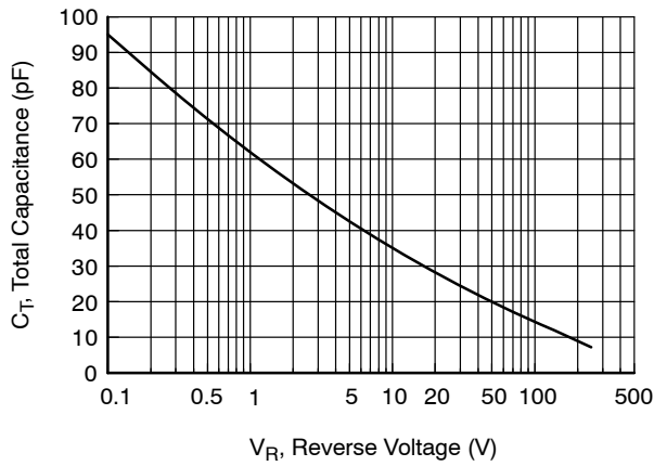
Figure 3. Total Capacitance
