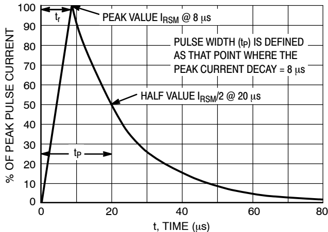
Figure 1. 8 x 20 \mu s Pulse Waveform
