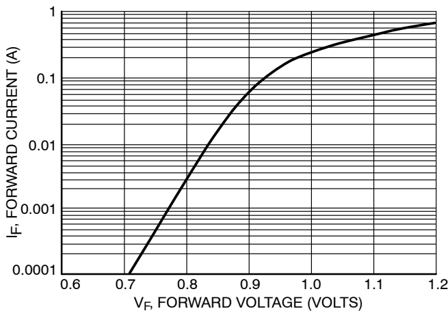
Figure 3. Forward Voltage
