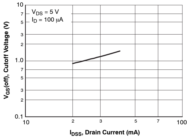
Figure 7. V_{GS(off)} - I_{DSS}
