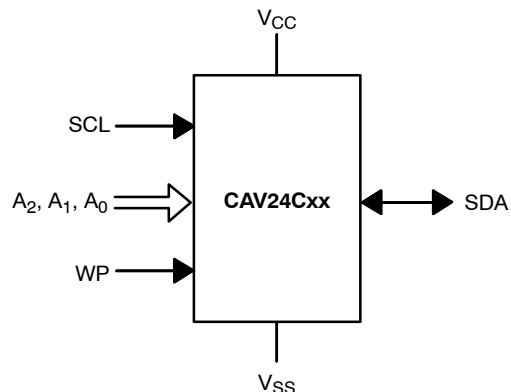
Figure 1. Functional Symbol
