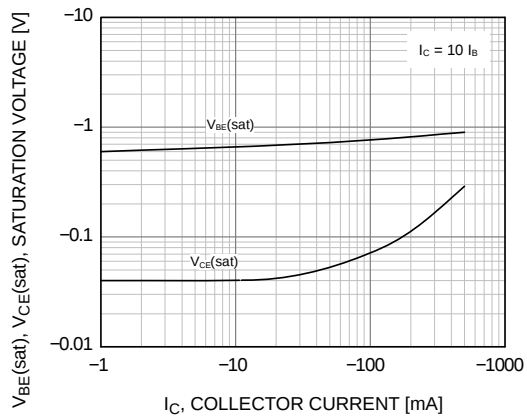
Figure 3. Base-Emmitter Saturation Voltage and Collector-Emmitter Saturation Voltage
