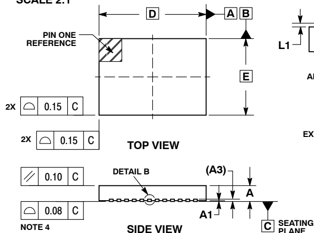
QFN40 7x5, 0.5P CASE 485EG ISSUE B
