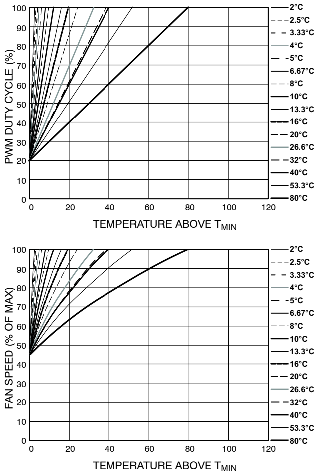
Figure 57. T RANGE and % Fan Speed Slopes with PWM MIN = 20%
