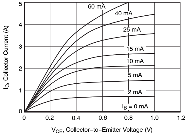
Figure 1. I_C - V_{CE}
