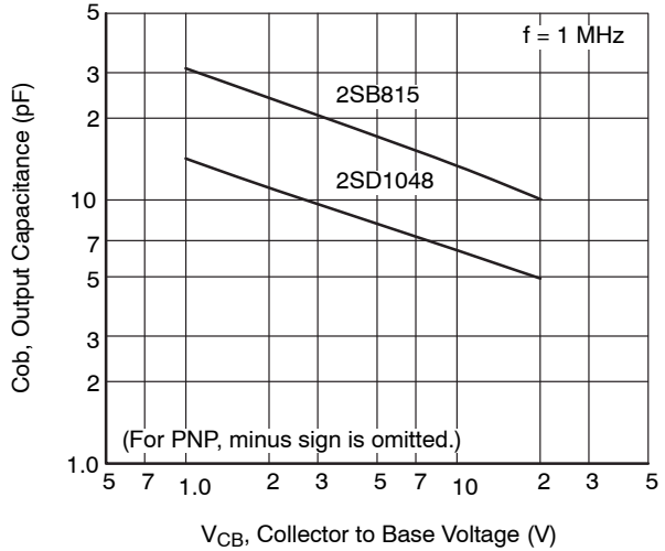
Figure 6. C_{ob} - V_{CB}
