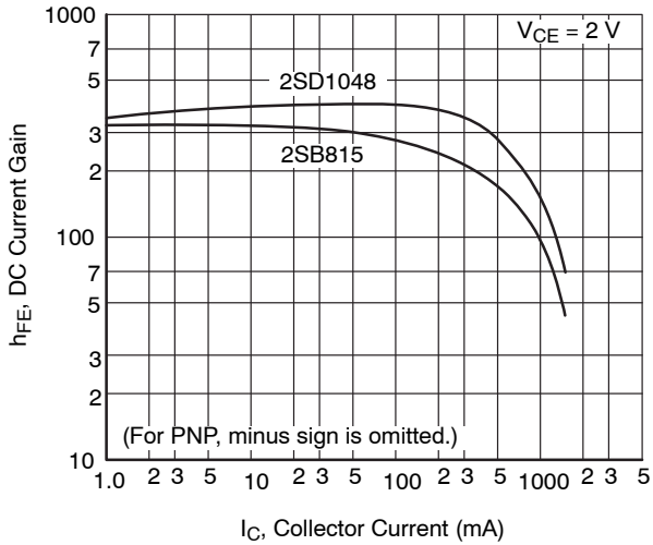
Figure 5. h_{FE} - I_C
