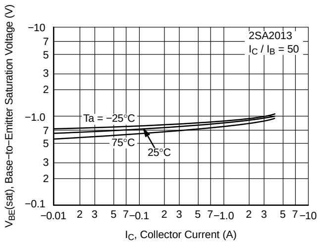
Figure 12. V_{BE(sat)} - I_C
