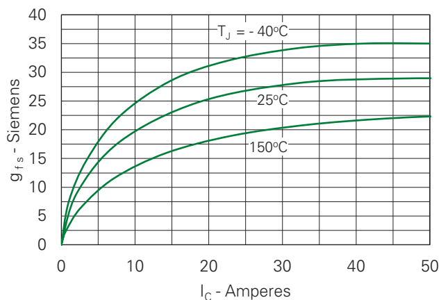
Fig. 7. Transconductance
