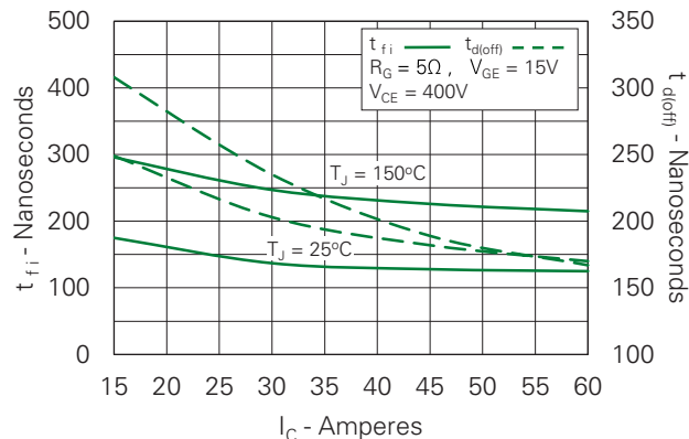
Fig. 16. Inductive Turn-off Switching Times vs. Collector Current
