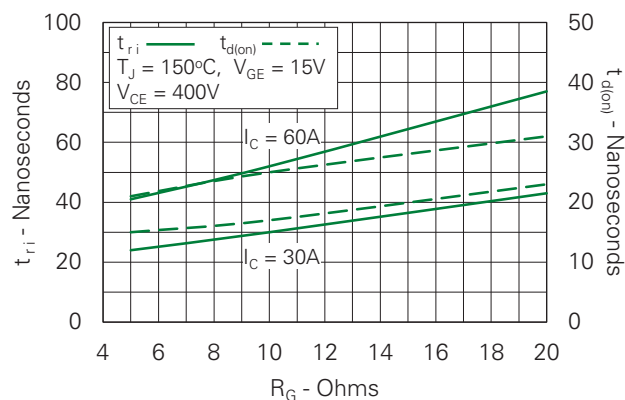
Fig. 18. Inductive Turn-on Switching Times vs. Gate Resistance
