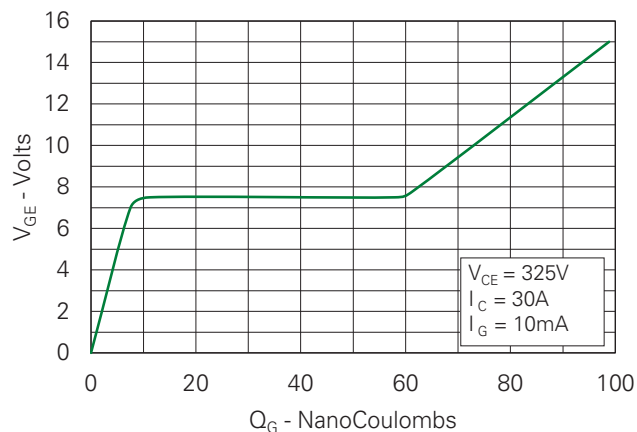
Fig. 8. Gate Charge
