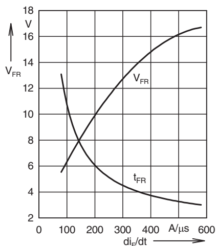
Fig. 15 Peak forward voltage versus -di_F/dt (Boost Diode)
