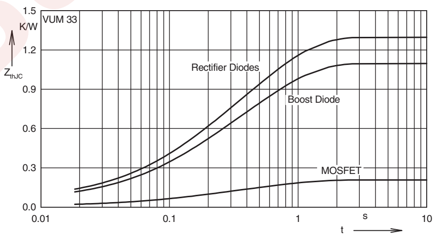
Fig. 19 Transient thermal impedance junction to case for all devices
