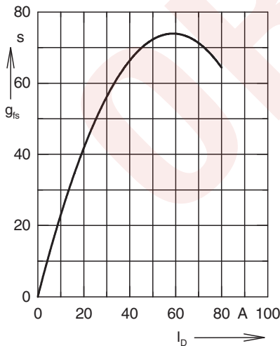
Fig. 9 Typ. transconductance, g_{is} = f(I_D) (MOSFET)
