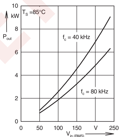
Fig. 17 Output power versus mains voltage
