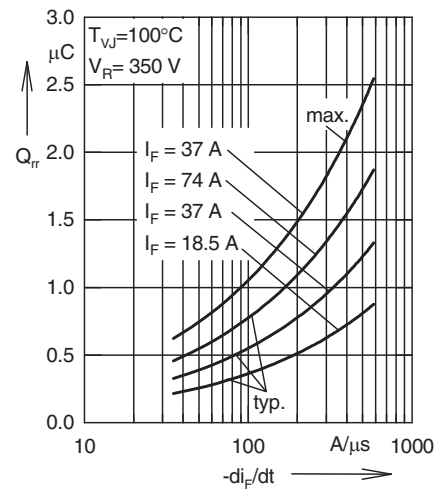
Fig. 11 Recovery charge versus -di_F/dt (Boost Diode)
