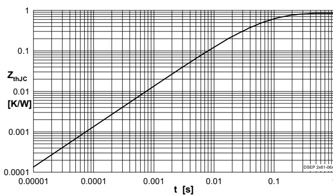
Fig. 7 Transient thermal resistance junction to case
