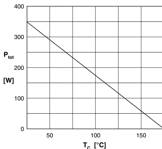
Fig. 4 Power derating
