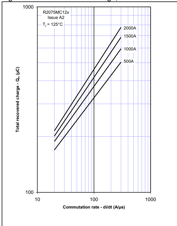
Figure 5 - Total recovered charge, Q_{rr}
