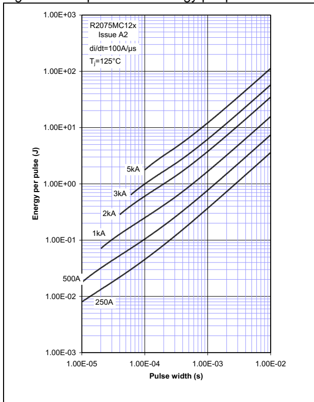
Figure 17 - Square wave energy per pulse
