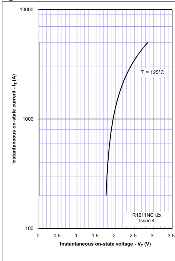
Figure 1 - On-state characteristics of Limit device
