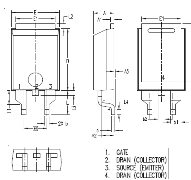
PLUS220SMD (IXTV_S) Outline
