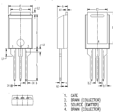
PLUS220 (IXTV) Outline
