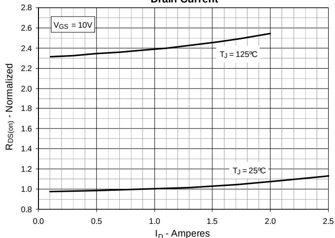
Fig. 4. R_{DS(on)} Normalized to I_D = 1A Value vs. Drain Current
