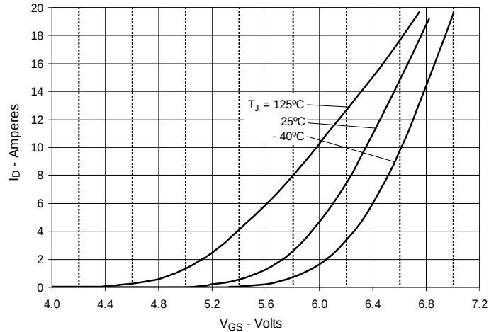
Fig. 6. Input Admittance
