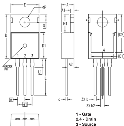
TO-220 Outline
