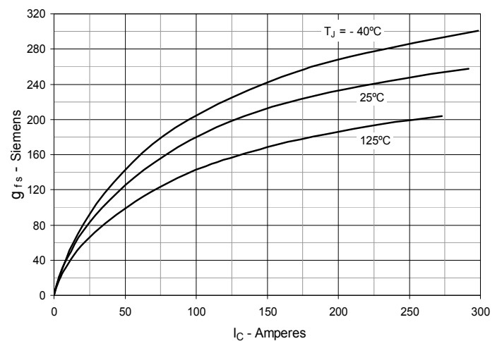
Fig. 6. Transconductance
