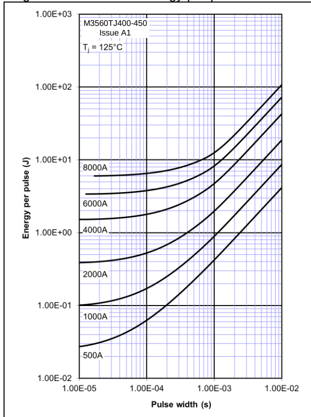
Figure 9 – Sine wave energy per pulse
