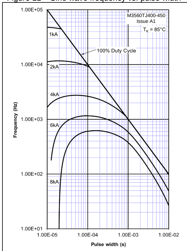
Figure 11 – Sine wave frequency vs. pulse width
