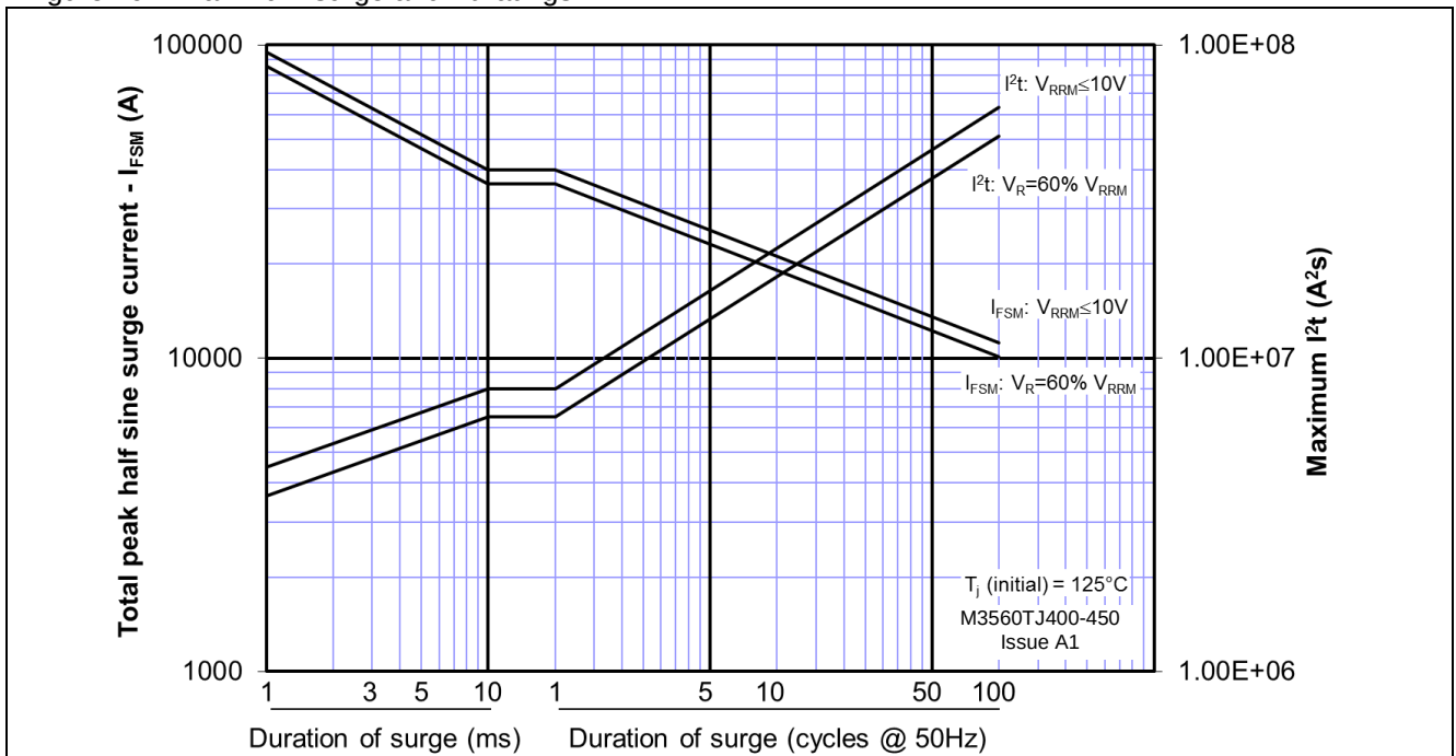
Figure 19 – Maximum surge and I^2t ratings
