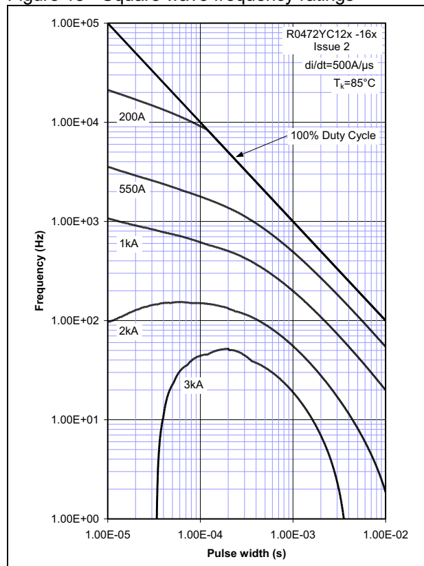
Figure 18 - Square wave frequency ratings
