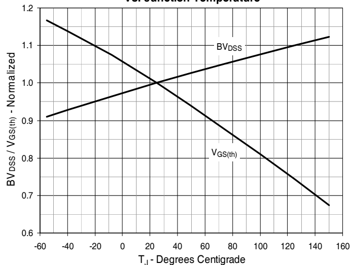
Fig. 6. Normalized Breakdown & Threshold Voltages vs. Junction Temperature
