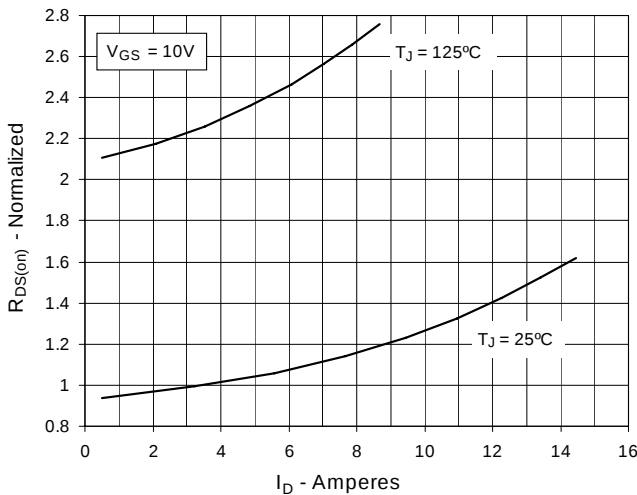
Fig. 5. R_{DS(on)} Normalized to I_D = 3.5\text{A} Value vs. Drain Current
