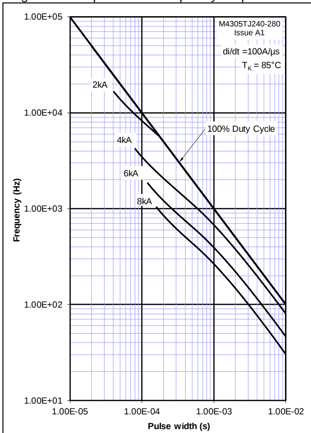
Figure 15 – Square wave frequency vs. pulse width
