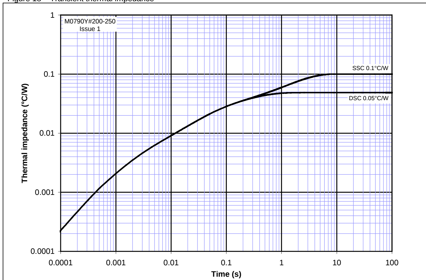
Figure 18 – Transient thermal impedance
