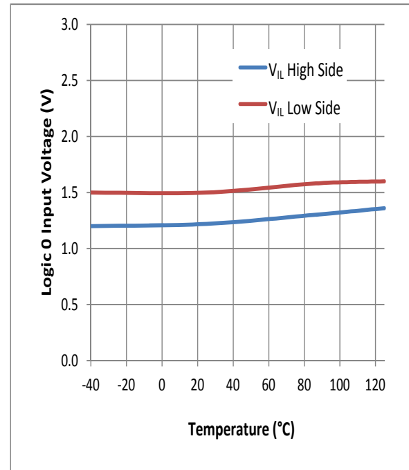
Figure 26. Logic 0 Input Voltage vs. Temperature
