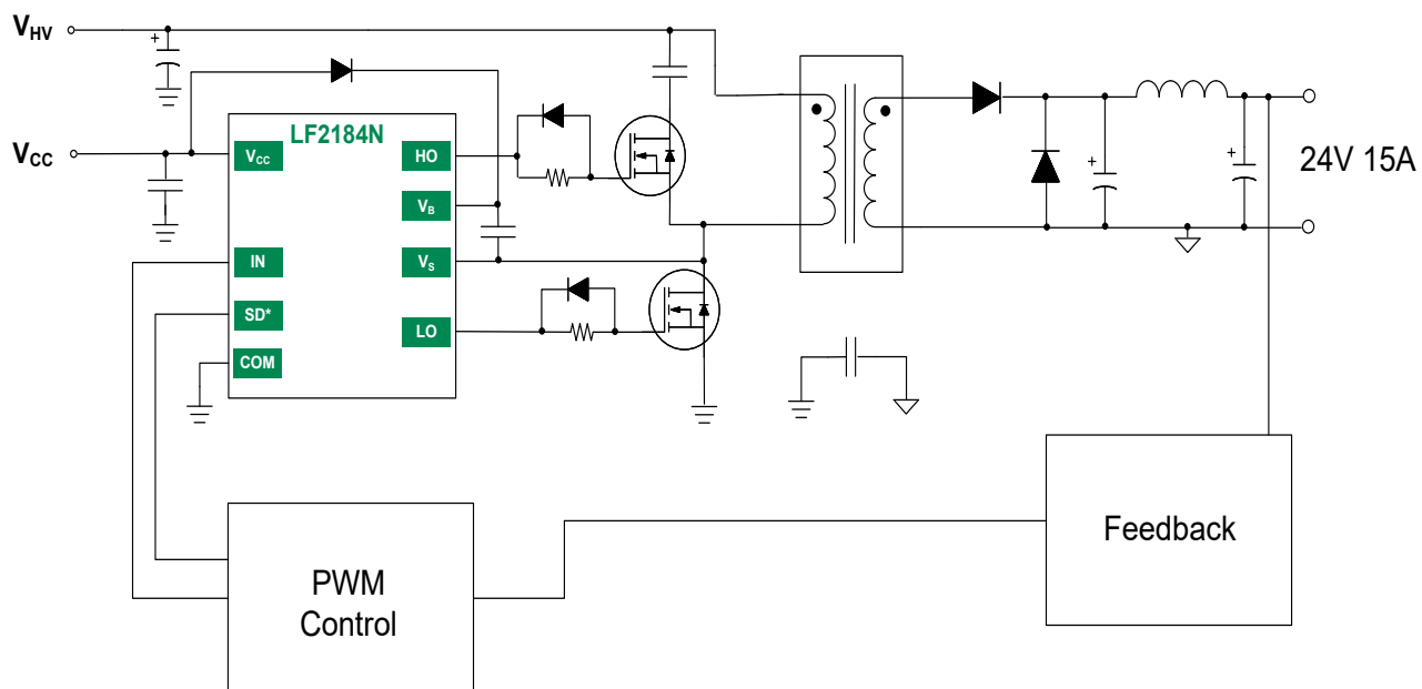
Figure 33. 360W Active Clamp Forward Converter using LF2184N
