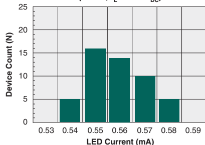
Typical I_F for Switch Operation (N=50, I_L=90\text{mA}_{DC} )
