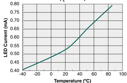
Typical I_F For Switch Dropout vs. Temperature ( I_L=80\text{mA} )
