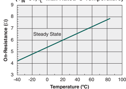
Typical On-Resistance vs. Temperature ( V_{IN}=0V , I_L =Max Rated @ Temperature)
