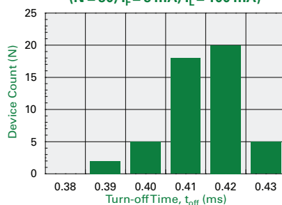
Typical Turn-off Time Distribution (N = 50, I_F = 5 mA, I_L = 100 mA)
