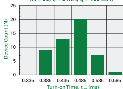
Typical Turn-on Time Distribution (N = 50, I_F = 5 mA, I_L = 100 mA)
