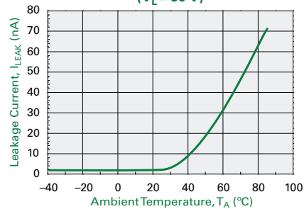
Typical Leakage Current vs. Temperature ( V_L = 60 \text{ V} )
