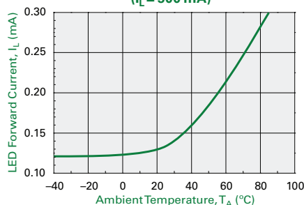
Typical LED Forward Current to Operate vs. Temperature ( I_L = 500 mA)
