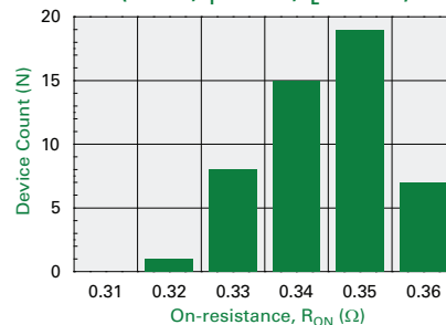
Typical On-resistance Distribution (N = 50, I_F = 2 mA, I_L = 0.75 A)
