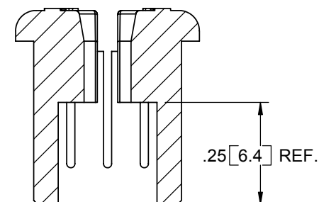
SECTION C-C SCALE 3 : 1
