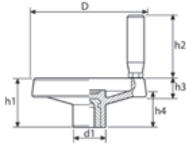
Type 2: With Handle
