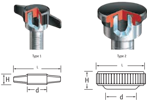
Knurled Knob (Type 2)
