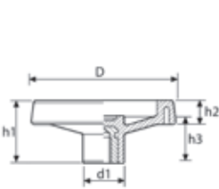
Type 1: Without Handle
