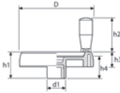
Type 2: With Folding Handle
