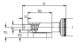
With Rest Position, with Knob
